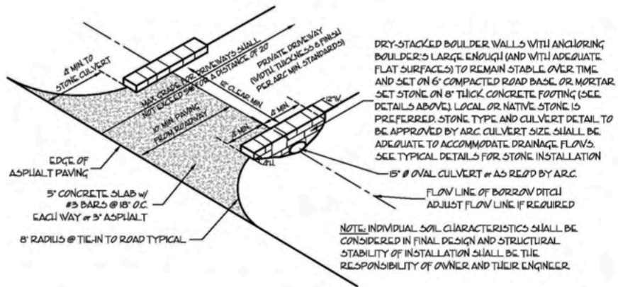
FIGURE 2: ISOMETRIC STONE CULVERT
